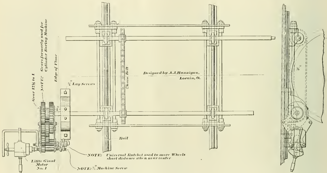
HANNIGAN'S ARRANGEMENT OF AIR VALVE-SETTING MECHANISM.
